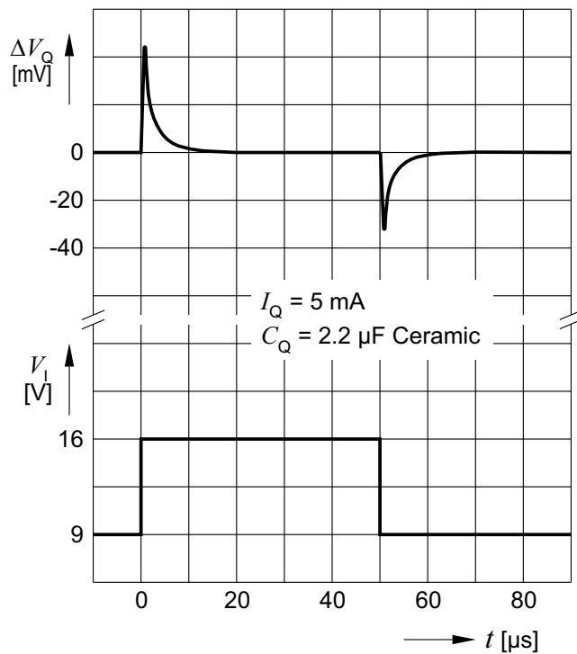
Line transient response
