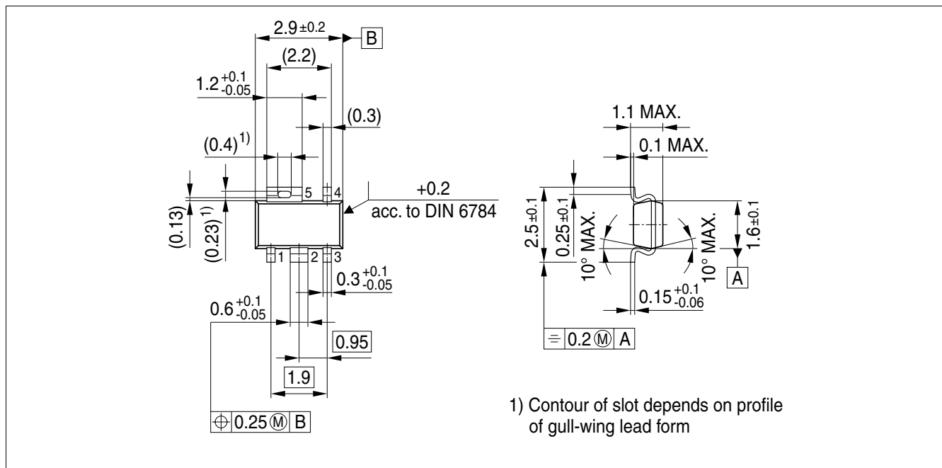
Figure 3 Outline PG-SCT595-5 1)
