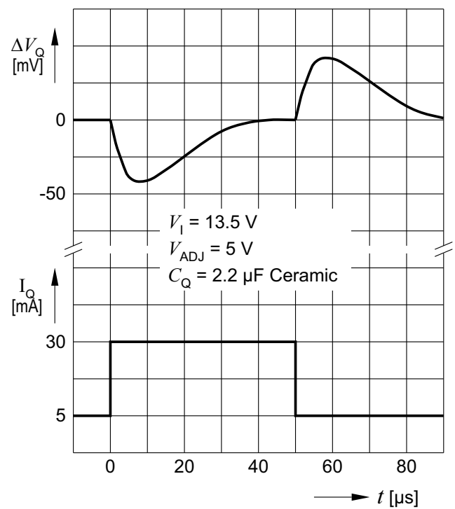
Load transient response
