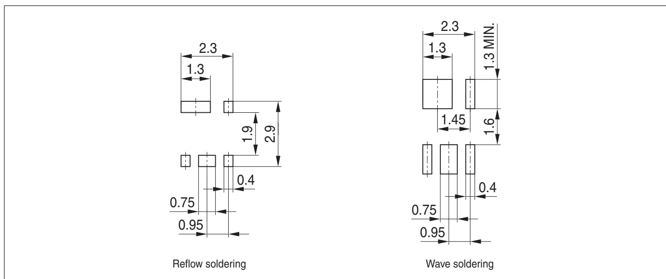
Figure 4 Footprint PG-SCT595-5 (Plastic dual small outline) 1)
