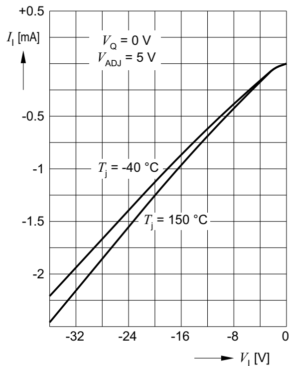
Reverse current I_I vs. input voltage V_I
